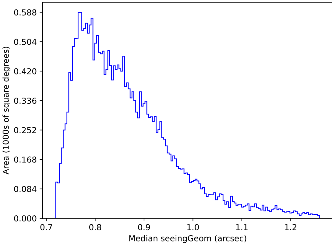
too_10_4v3.4_10yrs Yr 1 all bands: Median seeingGeom
