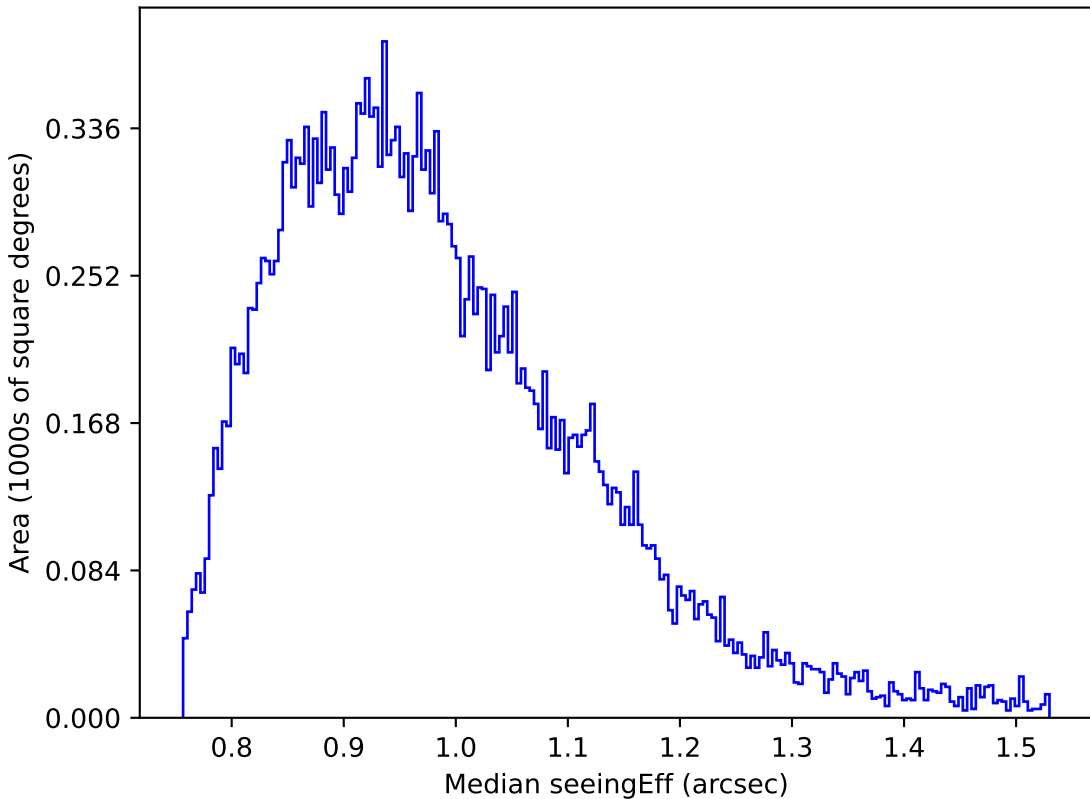
too_10_4v3.4_10yrs Yr 1 z band: Median seeingEff
