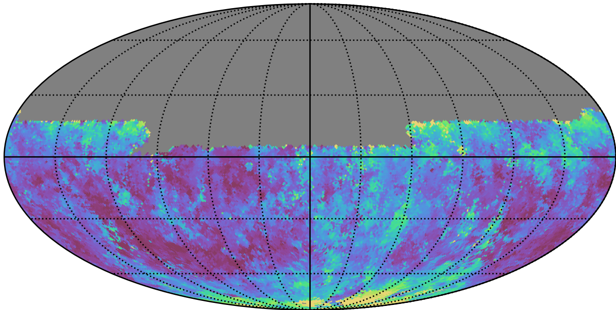
too_10_4v3.4_10yrs Yr 1 y band: Median seeingEff
