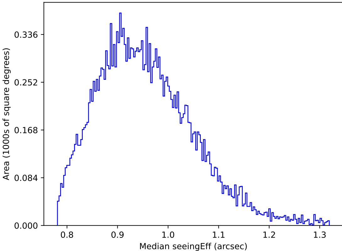
too_10_4v3.4_10yrs Yr 1 y band: Median seeingEff
