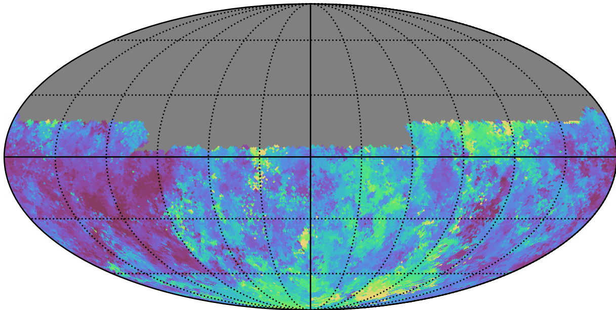
too_10_4v3.4_10yrs Yr 1 u band: Median seeingEff
