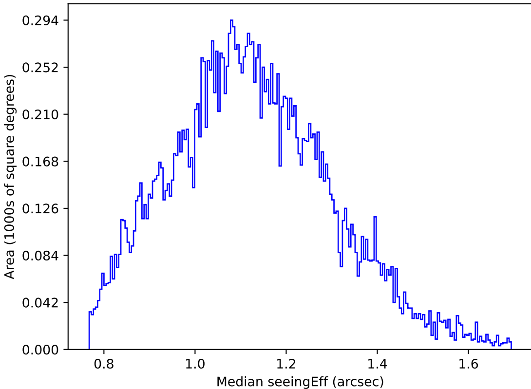
too_10_4v3.4_10yrs Yr 1 u band: Median seeingEff
