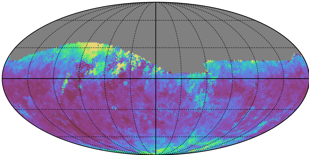
too_10_4v3.4_10yrs Yr 1 r band: Median seeingEff
