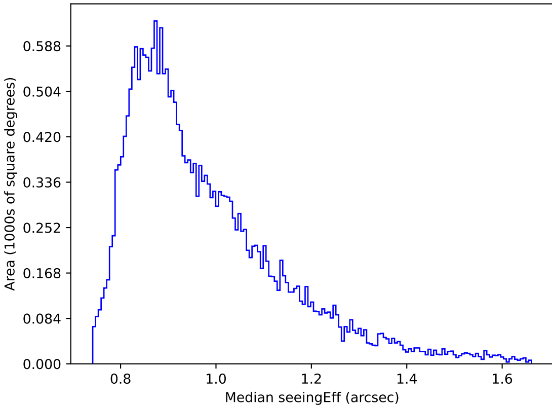
too_10_4v3.4_10yrs Yr 1 r band: Median seeingEff
