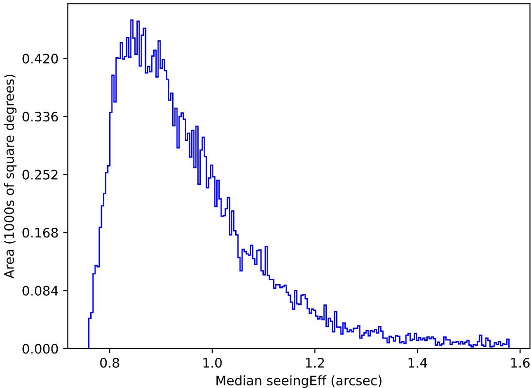
too_10_4v3.4_10yrs Yr 1 i band: Median seeingEff
