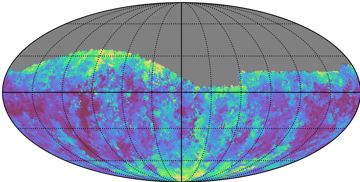
too_10_4v3.4_10yrs Yr 1 g band: Median seeingEff
