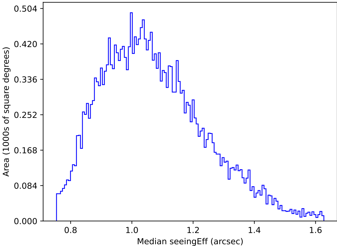
too_10_4v3.4_10yrs Yr 1 g band: Median seeingEff
