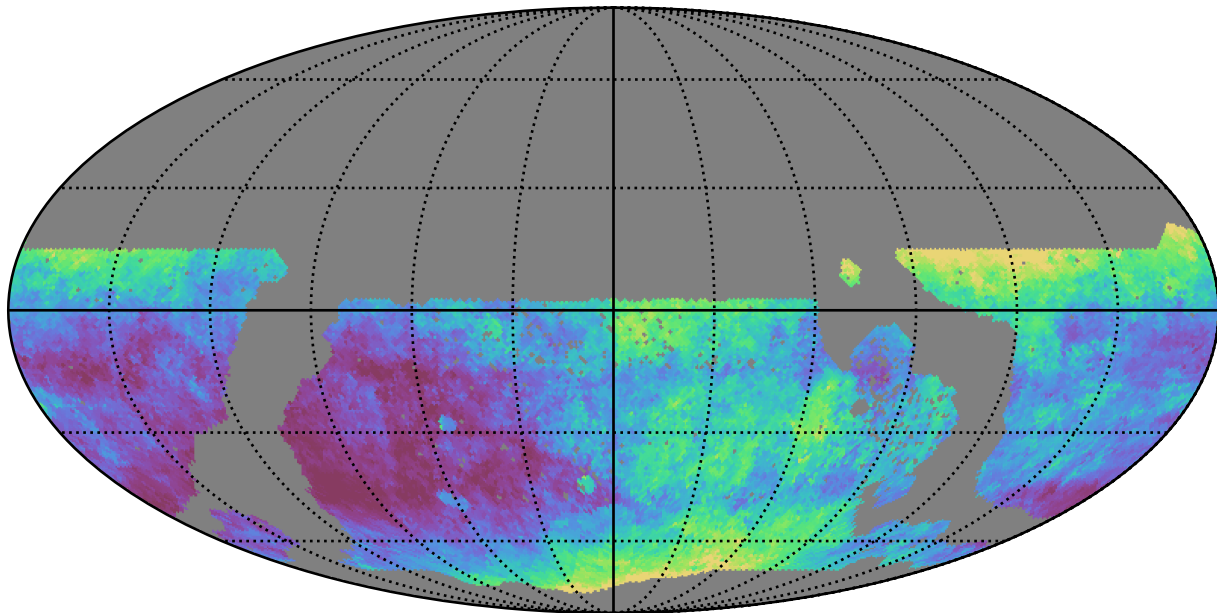
too_10_4v3.4_10yrs WFD z band: Median seeingEff
