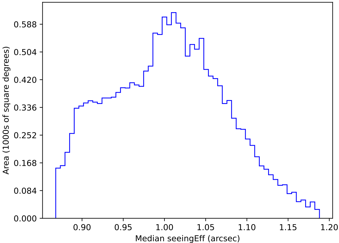
too_10_4v3.4_10yrs WFD z band: Median seeingEff
