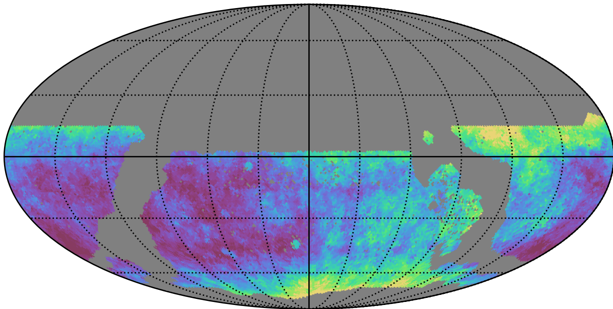
too_10_4v3.4_10yrs WFD y band: Median seeingEff
