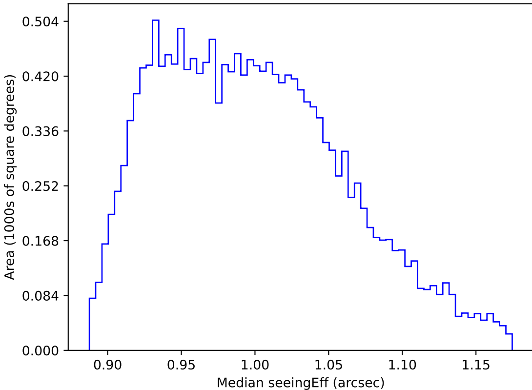
too_10_4v3.4_10yrs WFD y band: Median seeingEff
