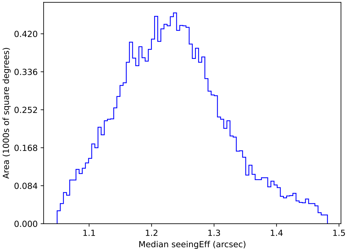
too_10_4v3.4_10yrs WFD u band: Median seeingEff
