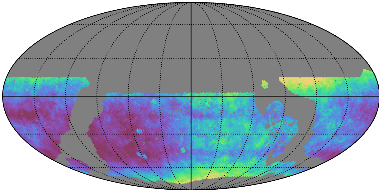
too_10_4v3.4_10yrs WFD i band: Median seeingEff
