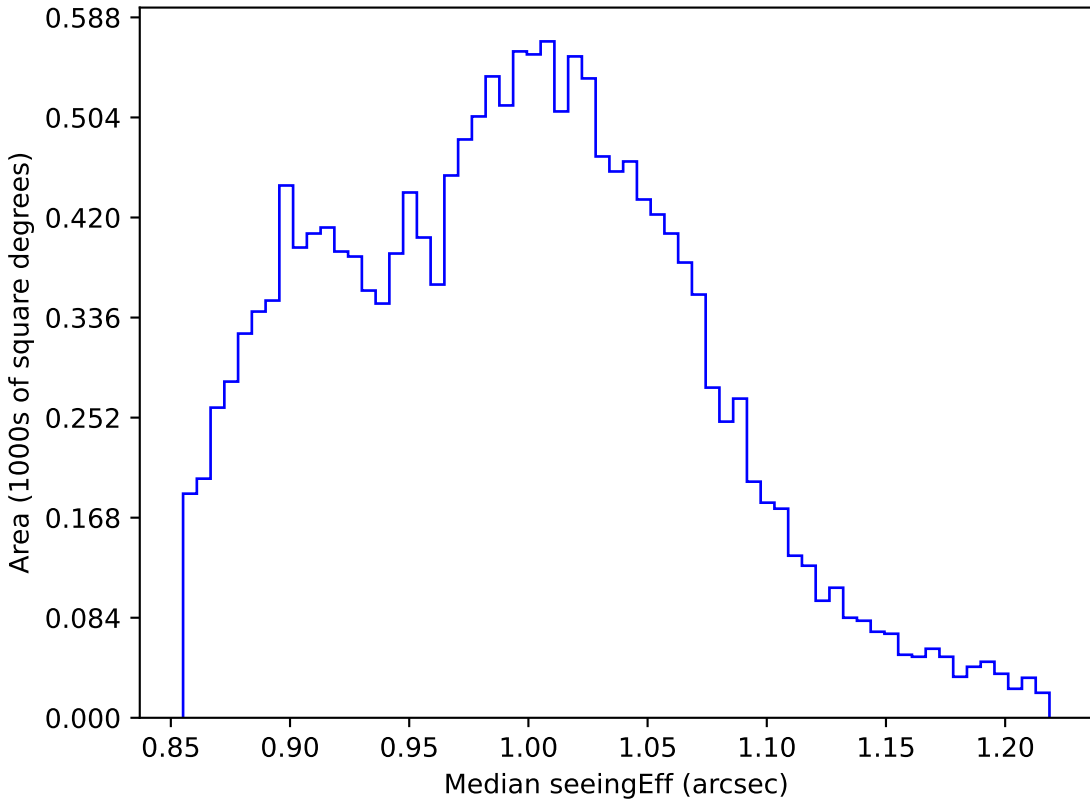
too_10_4v3.4_10yrs WFD i band: Median seeingEff
