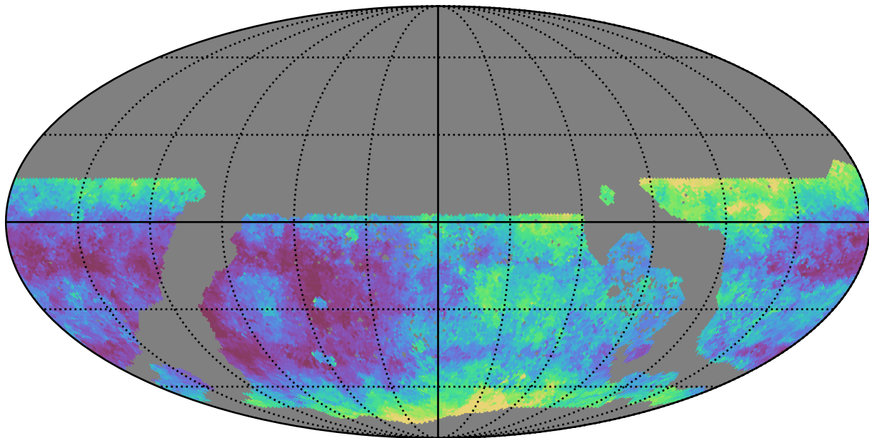
too_10_4v3.4_10yrs WFD g band: Median seeingEff
