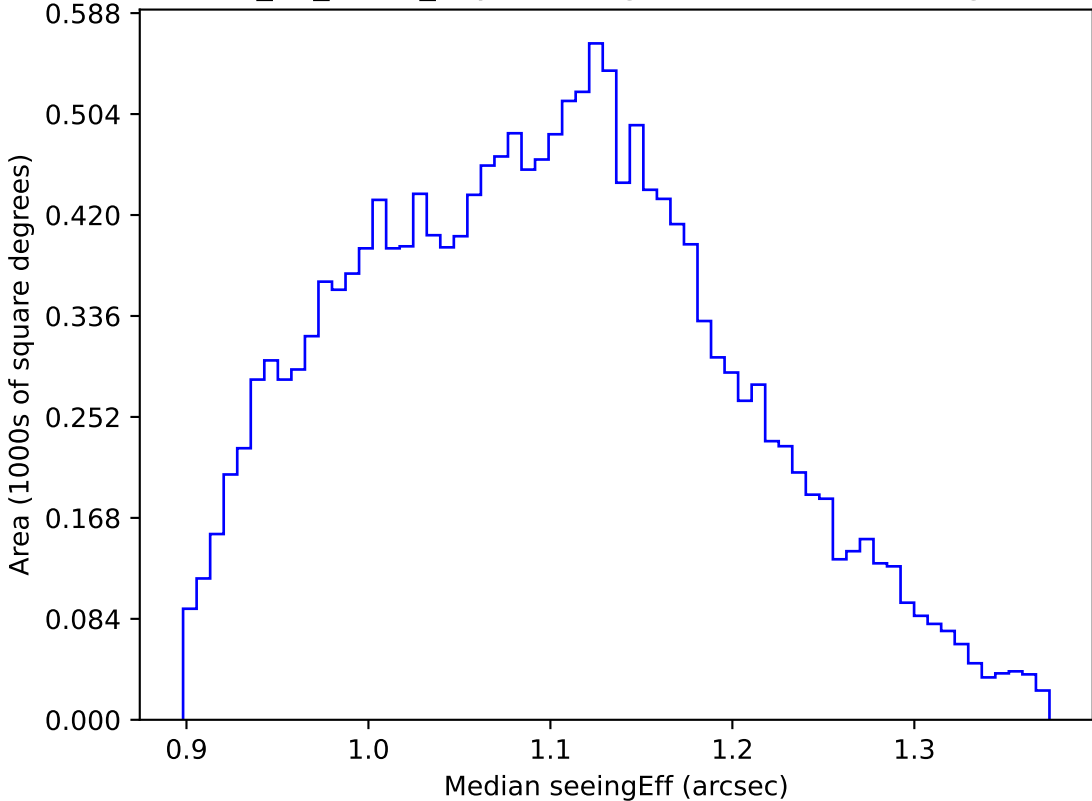
too_10_4v3.4_10yrs WFD g band: Median seeingEff
