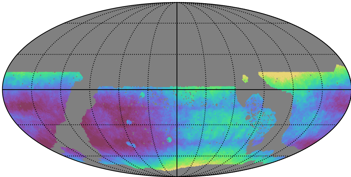
too_10_4v3.4_10yrs WFD all bands: Median seeingEff
