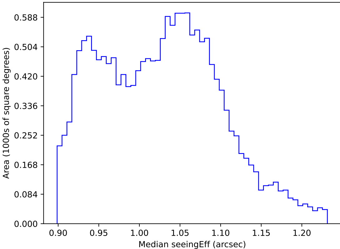
too_10_4v3.4_10yrs WFD all bands: Median seeingEff
