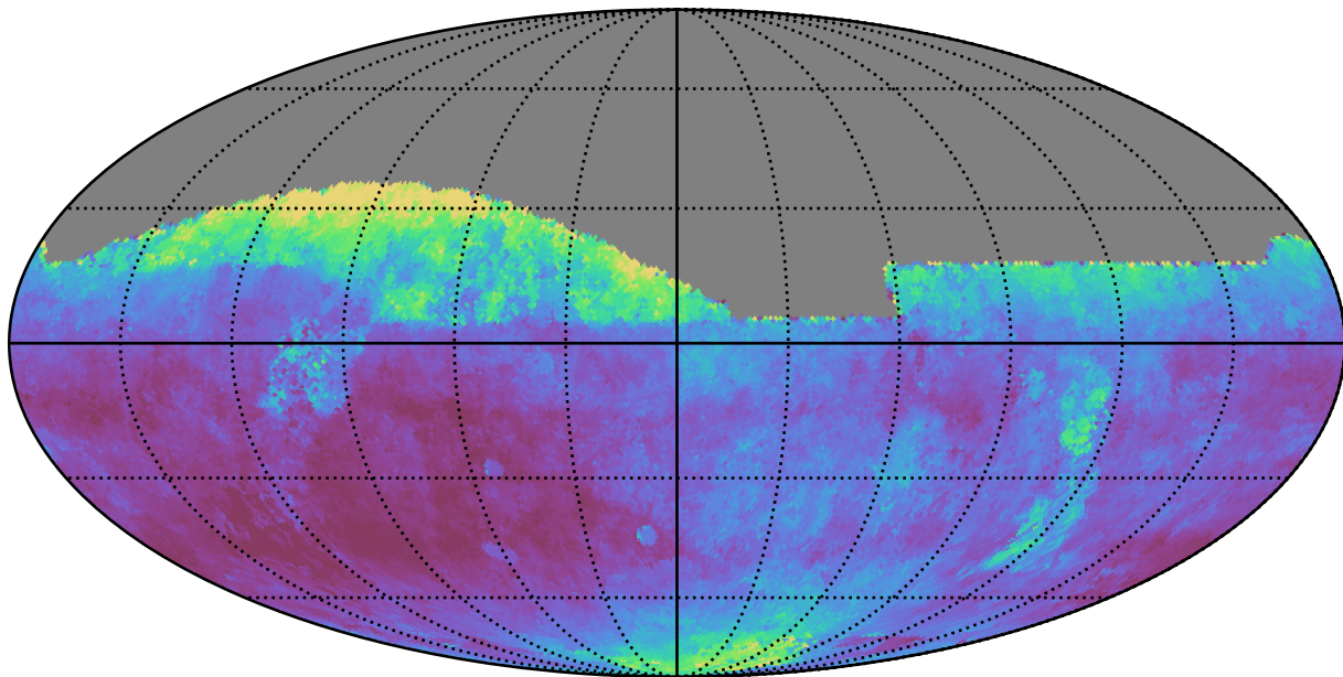
too_10_4v3.4_10yrs All sky z band: Median seeingEff
