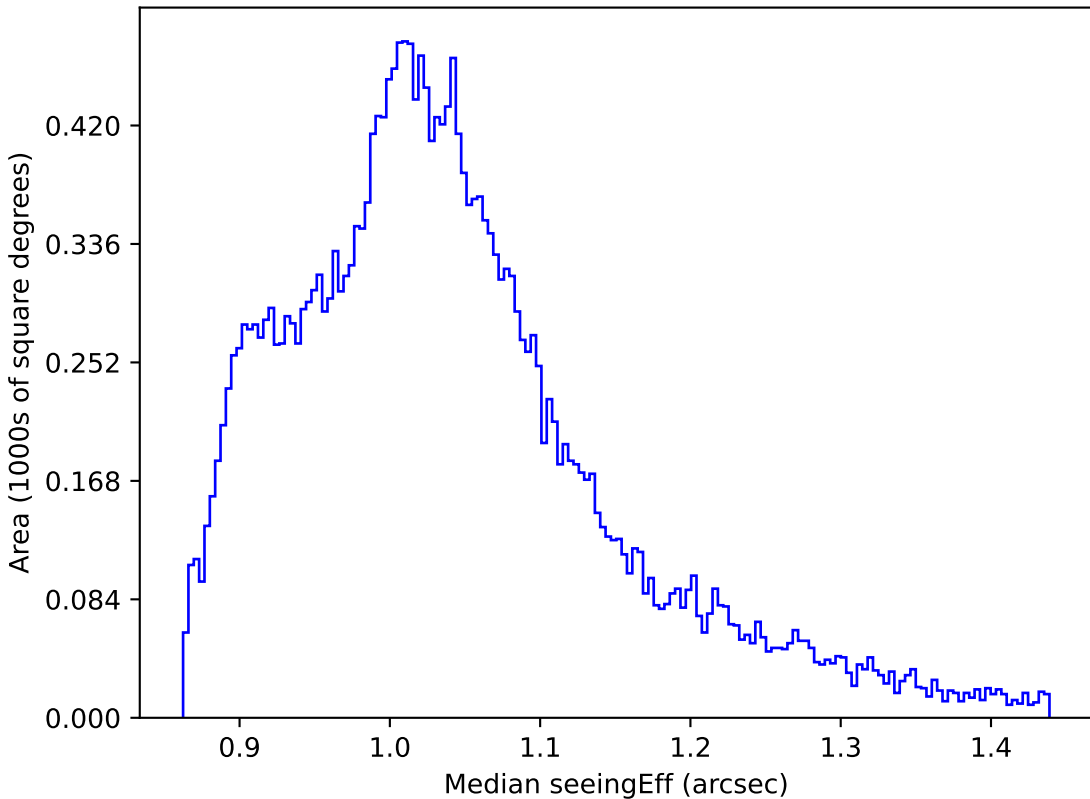
too_10_4v3.4_10yrs All sky z band: Median seeingEff
