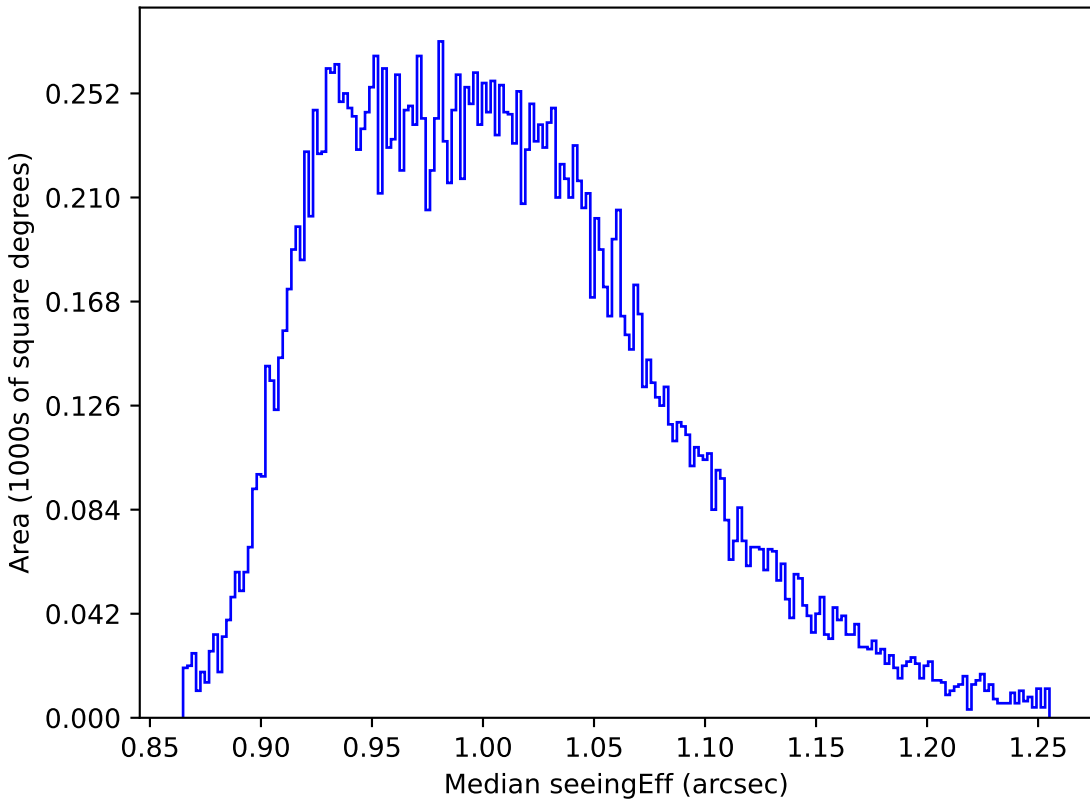
too_10_4v3.4_10yrs All sky y band: Median seeingEff
