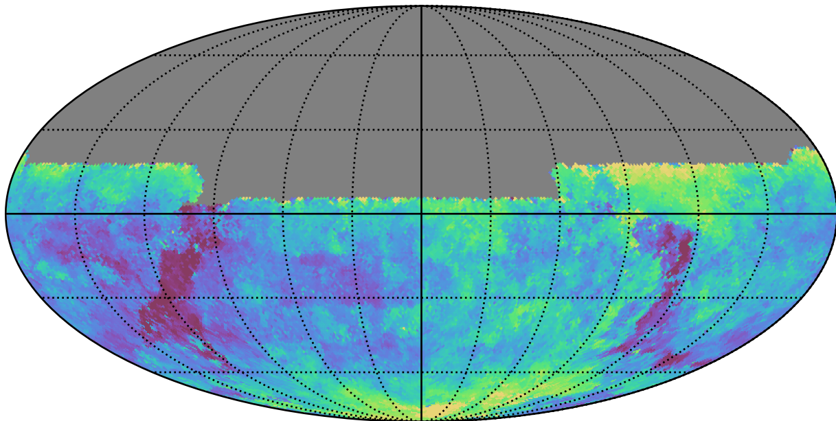
too_10_4v3.4_10yrs All sky u band: Median seeingEff
