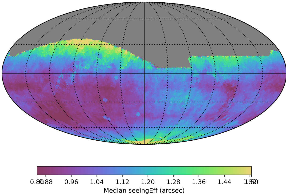
too_10_4v3.4_10yrs All sky r band: Median seeingEff
