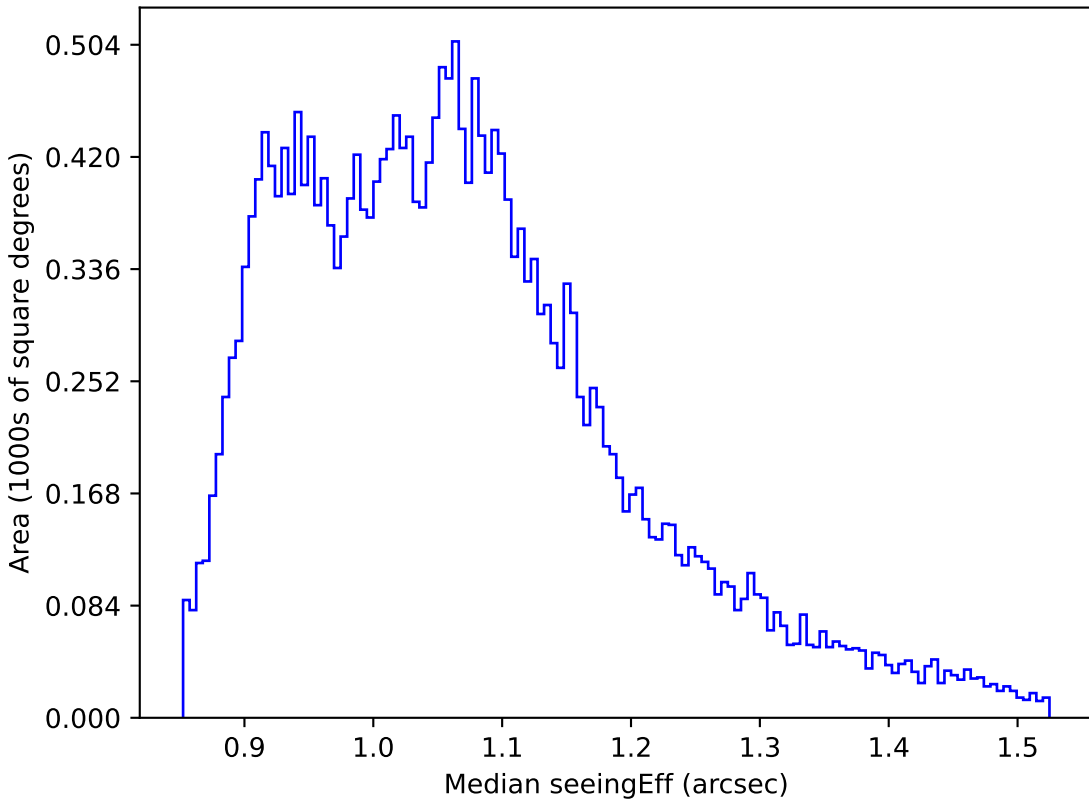
too_10_4v3.4_10yrs All sky r band: Median seeingEff
