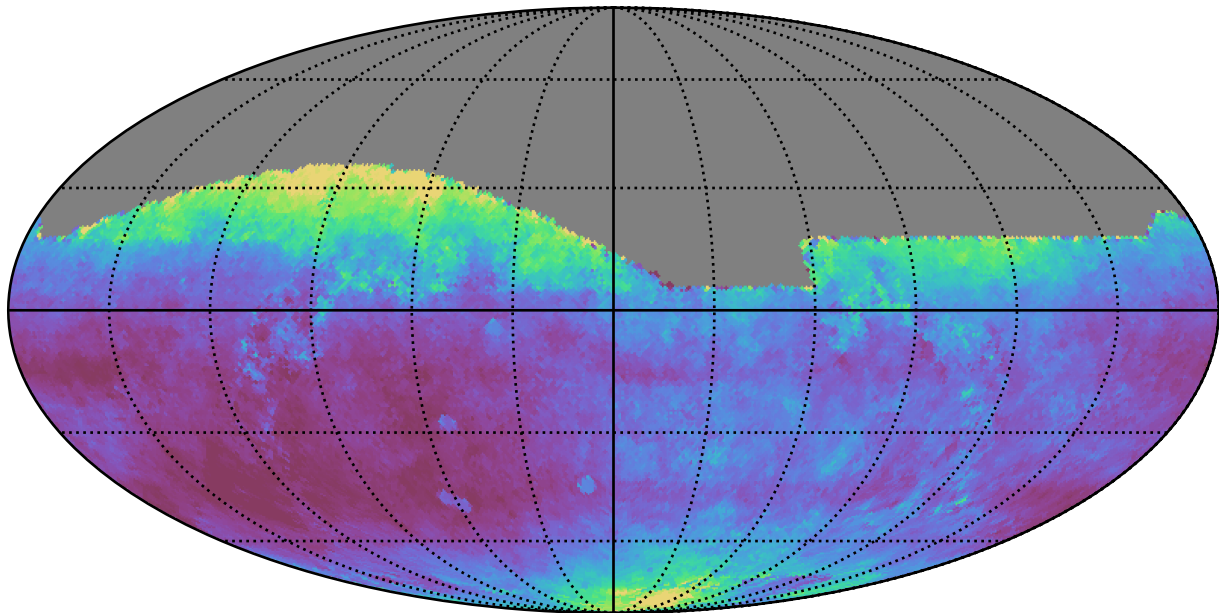
too_10_4v3.4_10yrs All sky i band: Median seeingEff
