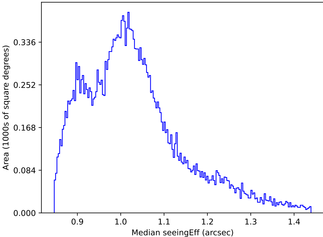
too_10_4v3.4_10yrs All sky i band: Median seeingEff
