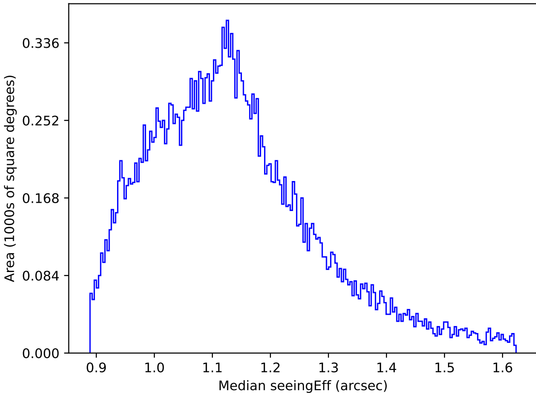
too_10_4v3.4_10yrs All sky g band: Median seeingEff
