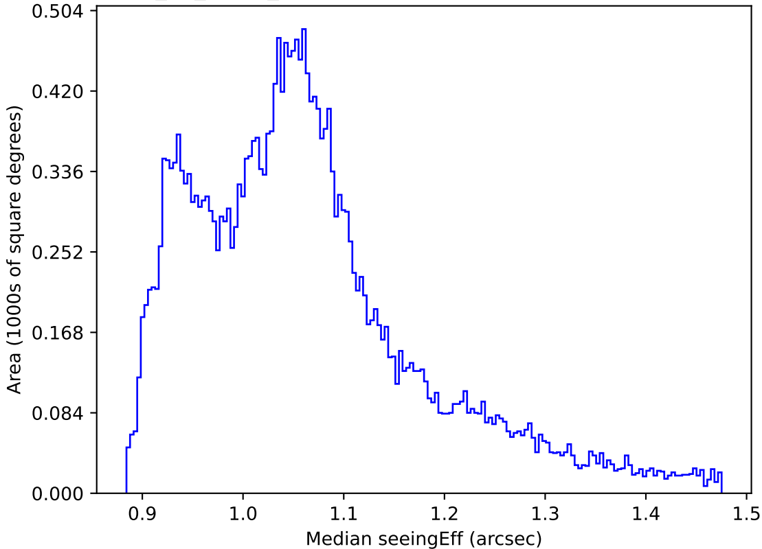
too_10_4v3.4_10yrs All sky all bands: Median seeingEff
