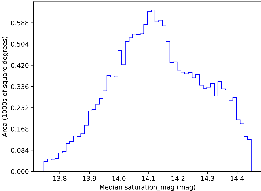
too_10_4v3.4_10yrs WFD z band: Median saturation_mag
