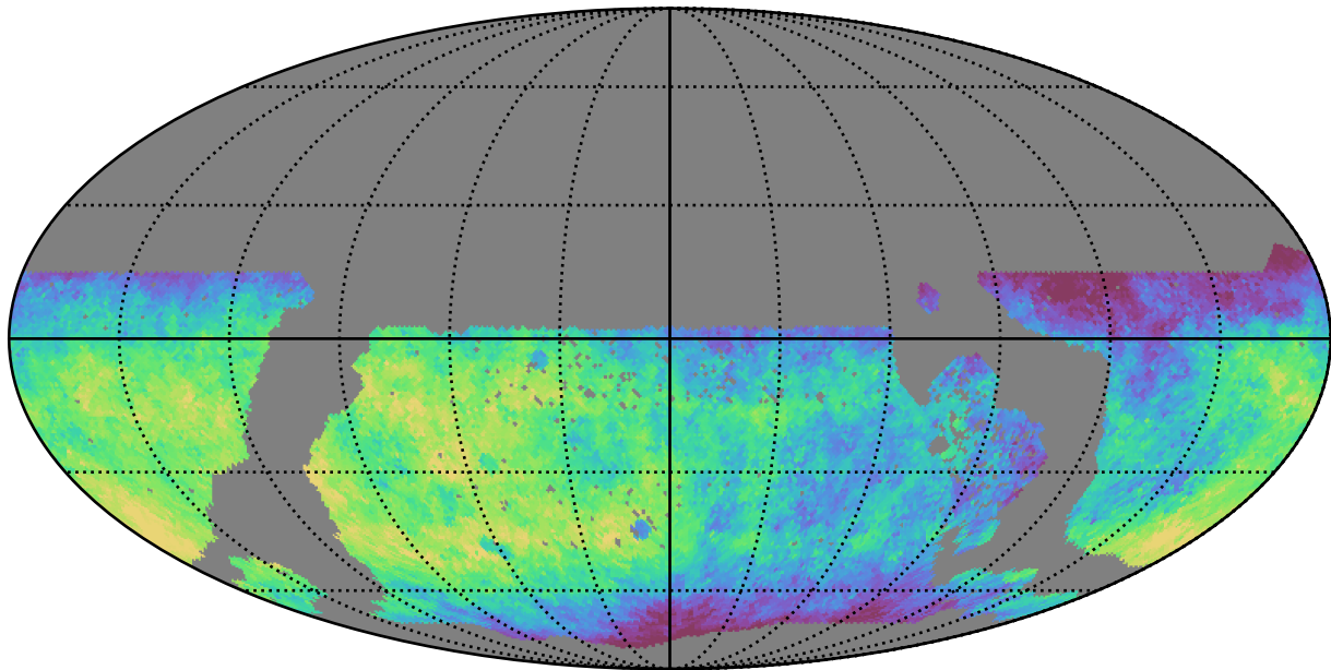
too_10_4v3.4_10yrs WFD y band: Median saturation_mag
