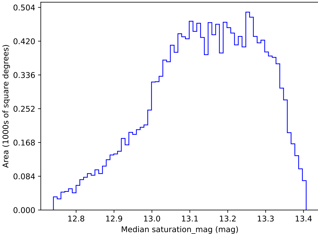
too_10_4v3.4_10yrs WFD y band: Median saturation_mag
