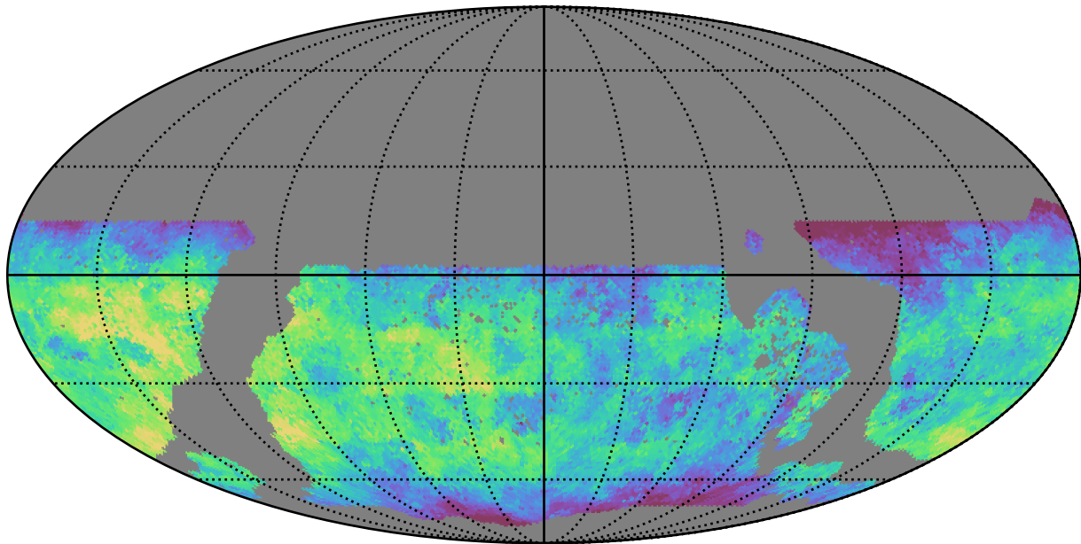
too_10_4v3.4_10yrs WFD u band: Median saturation_mag
