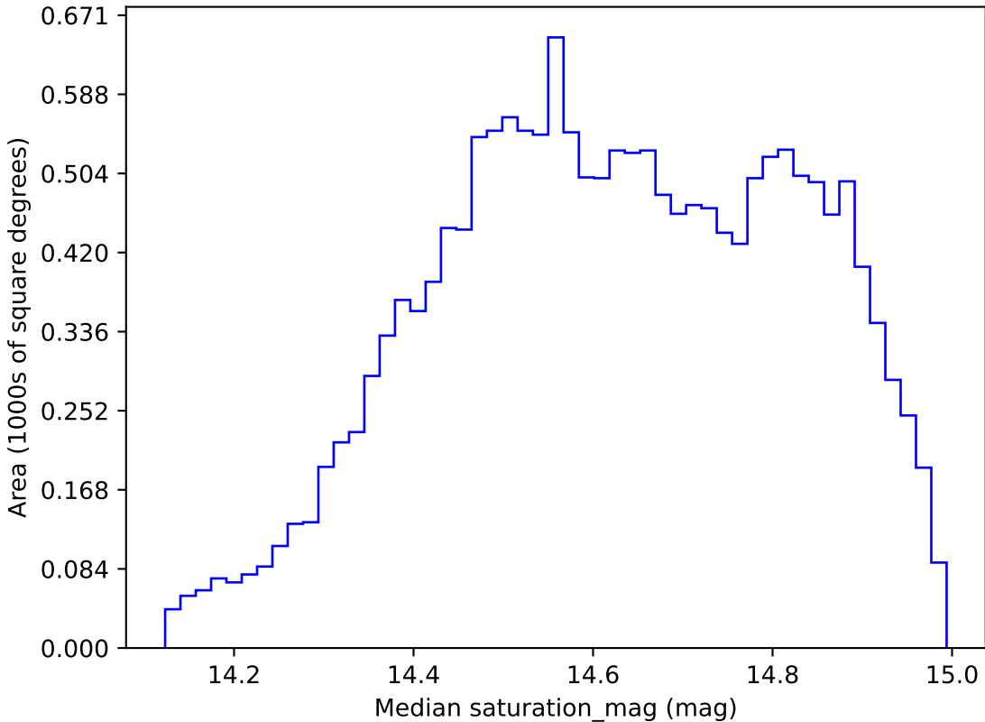
too_10_4v3.4_10yrs WFD r band: Median saturation_mag
