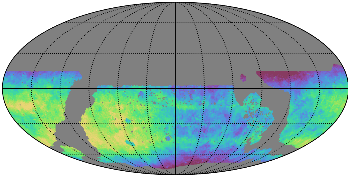
too_10_4v3.4_10yrs WFD i band: Median saturation_mag
