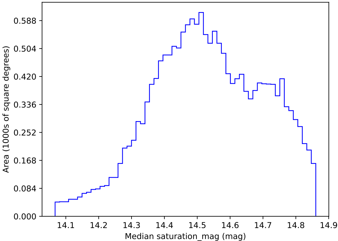
too_10_4v3.4_10yrs WFD i band: Median saturation_mag
