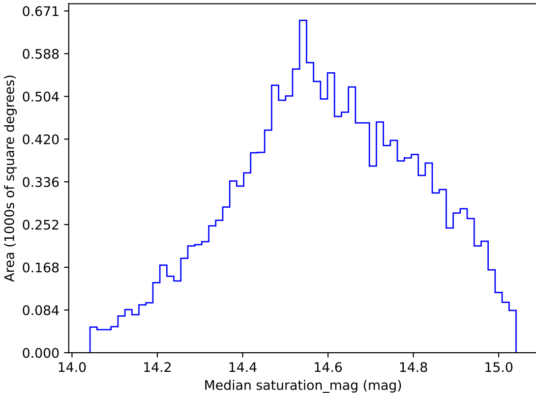
too_10_4v3.4_10yrs WFD g band: Median saturation_mag
