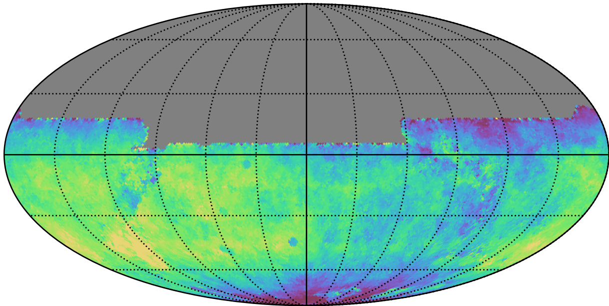
too_10_4v3.4_10yrs All sky y band: Median saturation_mag
