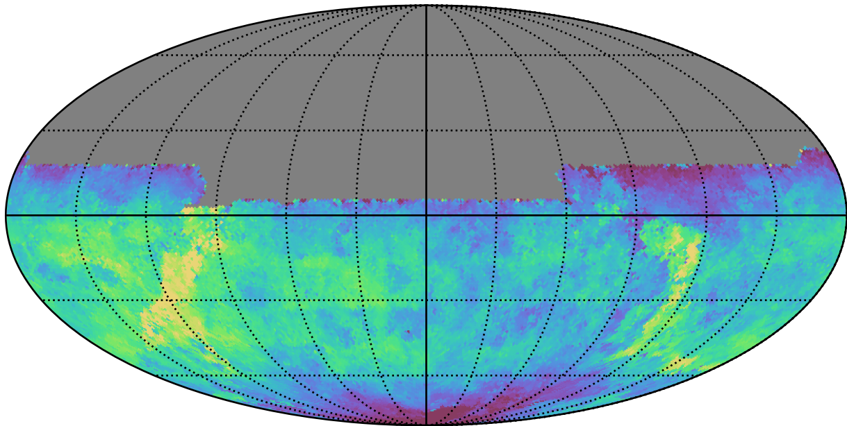
too_10_4v3.4_10yrs All sky u band: Median saturation_mag
