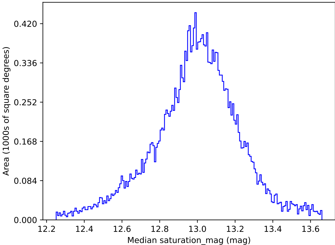
too_10_4v3.4_10yrs All sky u band: Median saturation_mag
