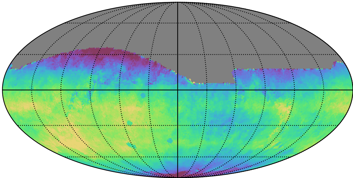
too_10_4v3.4_10yrs All sky r band: Median saturation_mag
