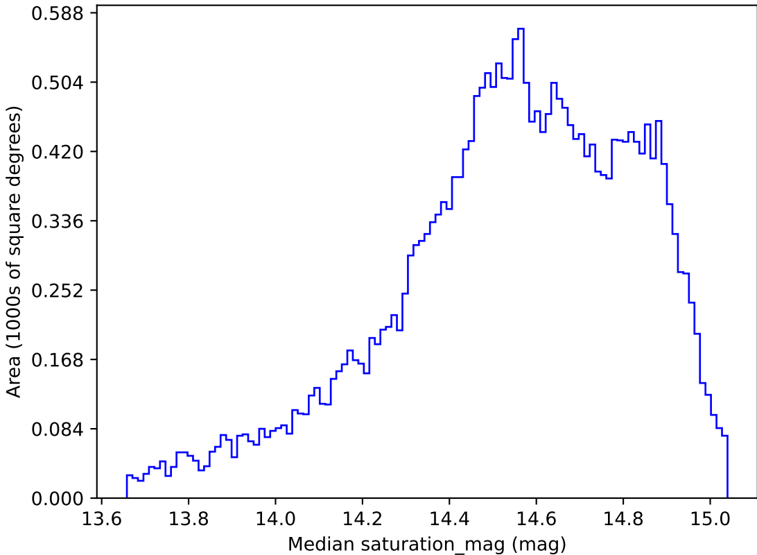
too_10_4v3.4_10yrs All sky r band: Median saturation_mag
