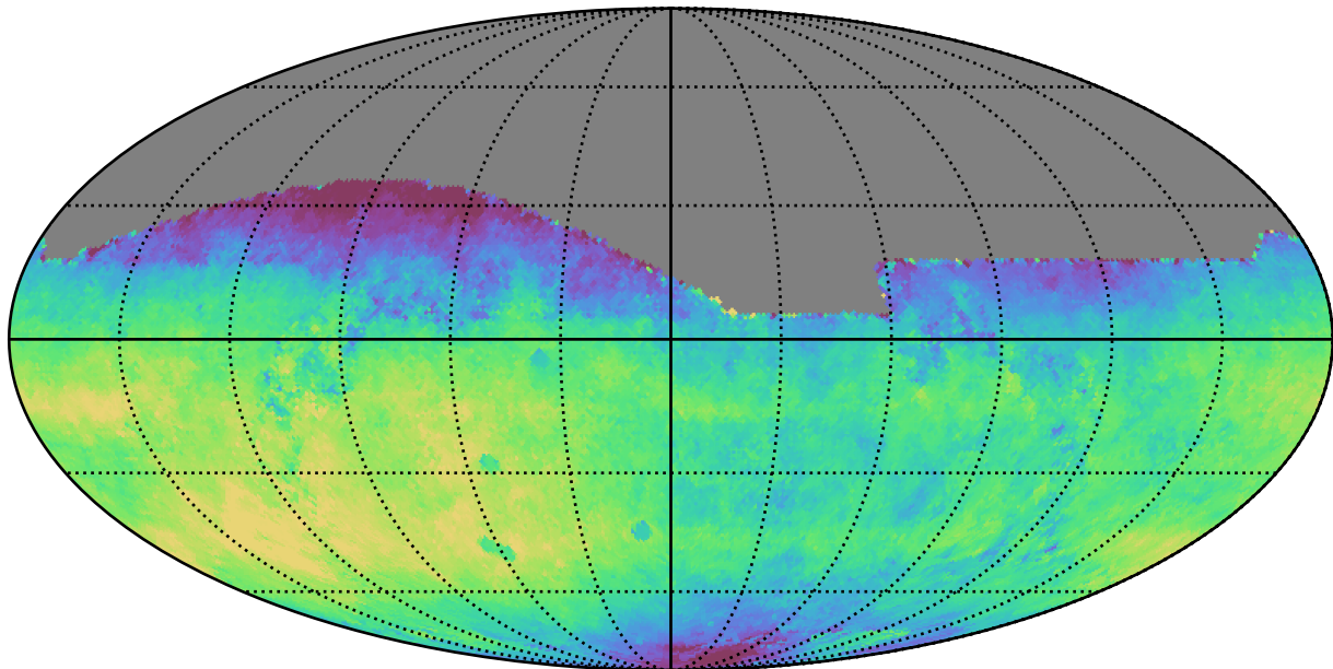
too_10_4v3.4_10yrs All sky i band: Median saturation_mag
