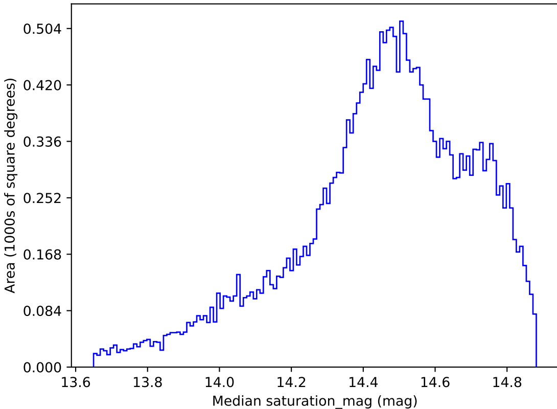
too_10_4v3.4_10yrs All sky i band: Median saturation_mag
