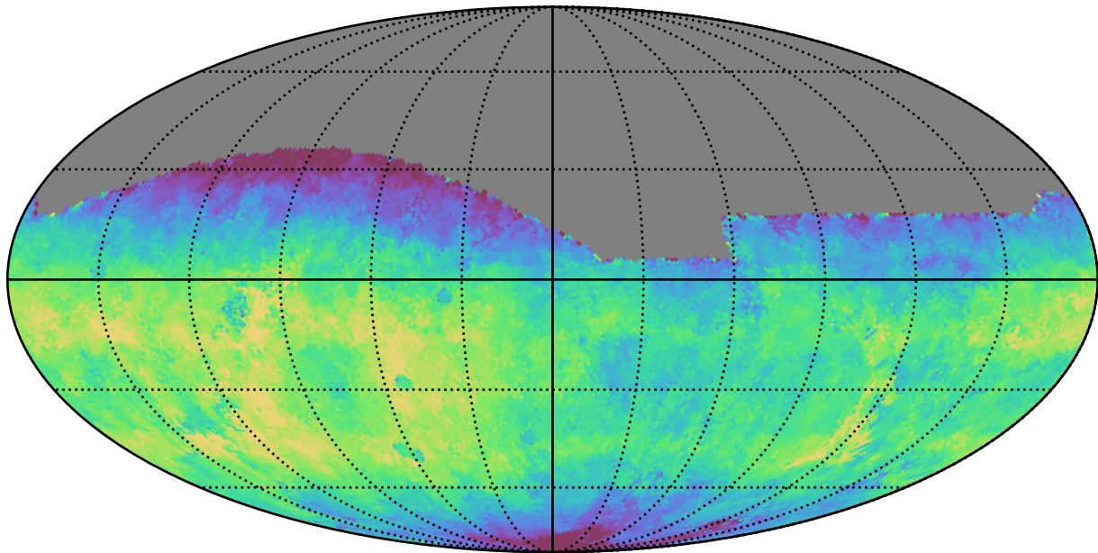
too_10_4v3.4_10yrs All sky g band: Median saturation_mag
