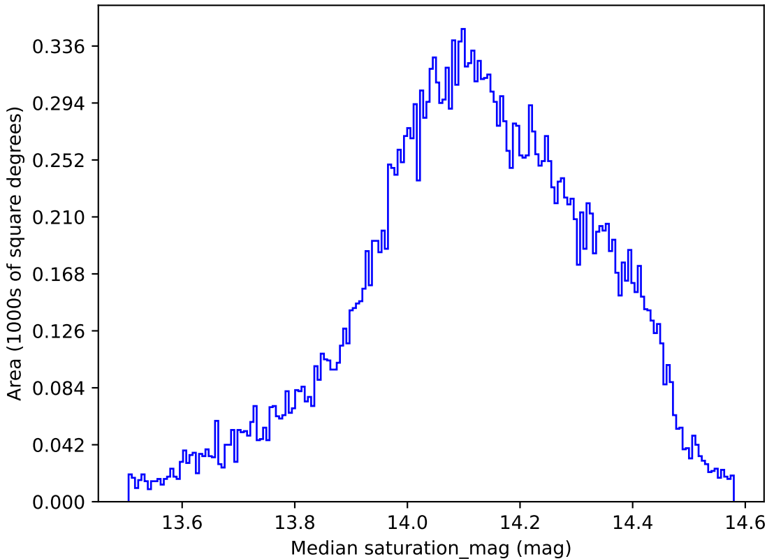
too_10_4v3.4_10yrs All sky all bands: Median saturation_mag
