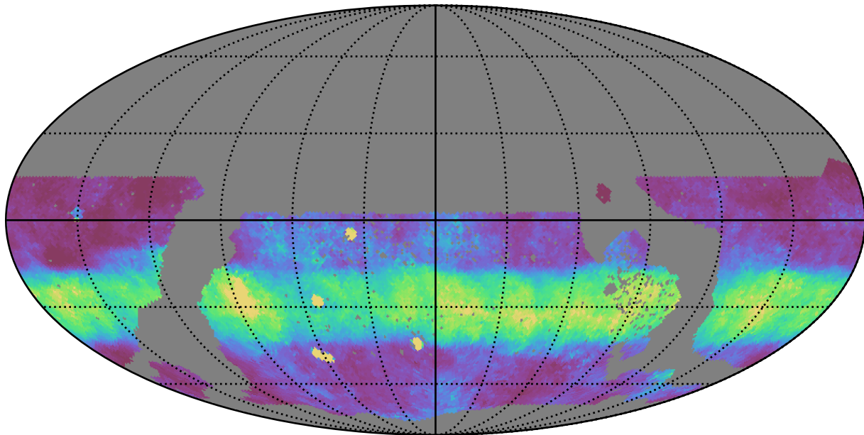
too_10_4v3.4_10yrs WFD z band: Median normairmass
